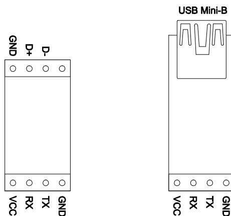
Board Pinout
